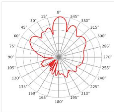
Elevation @ 5.8GHz
