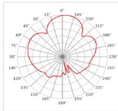
Azimuth @ 5.8GHz
